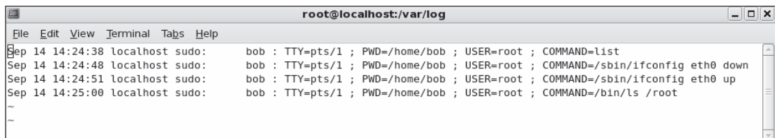
Figure 2.20 Sudo Log File Displaying User Bob's Commands
