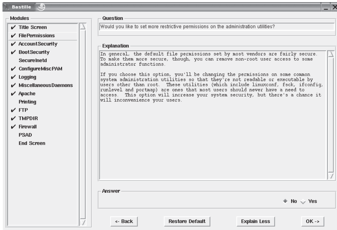
Figure 2.11 Bastille Linux Question-and-Answer Wizard
