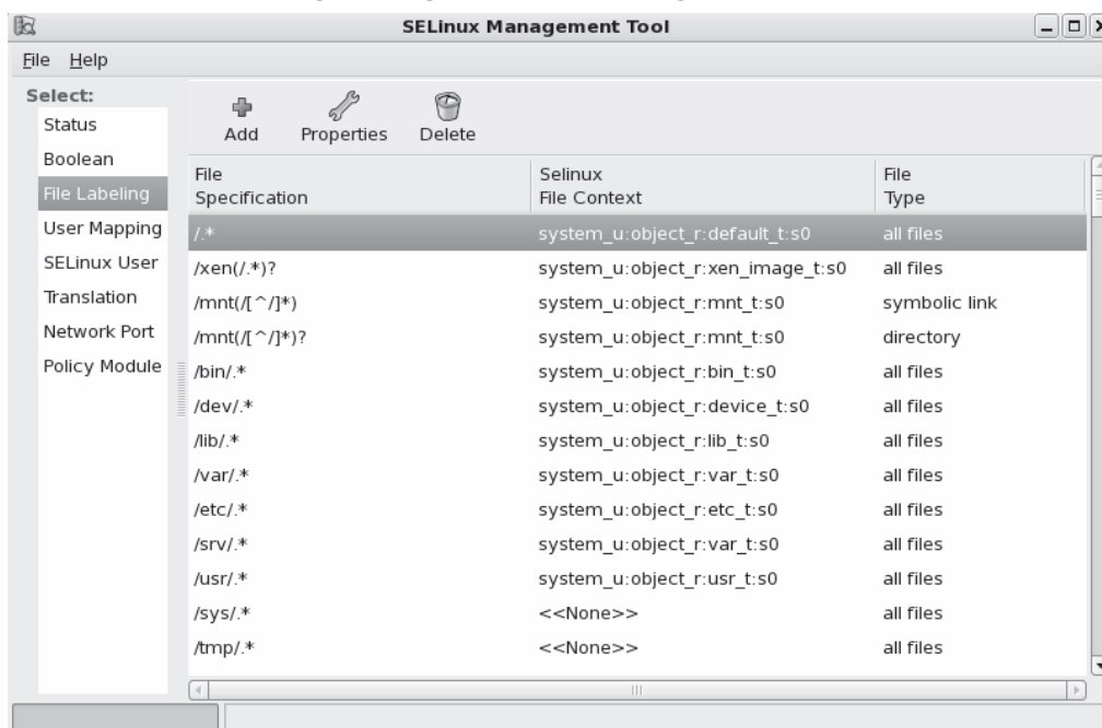
Figure 2.28 File Labeling through SELinux Management tool
